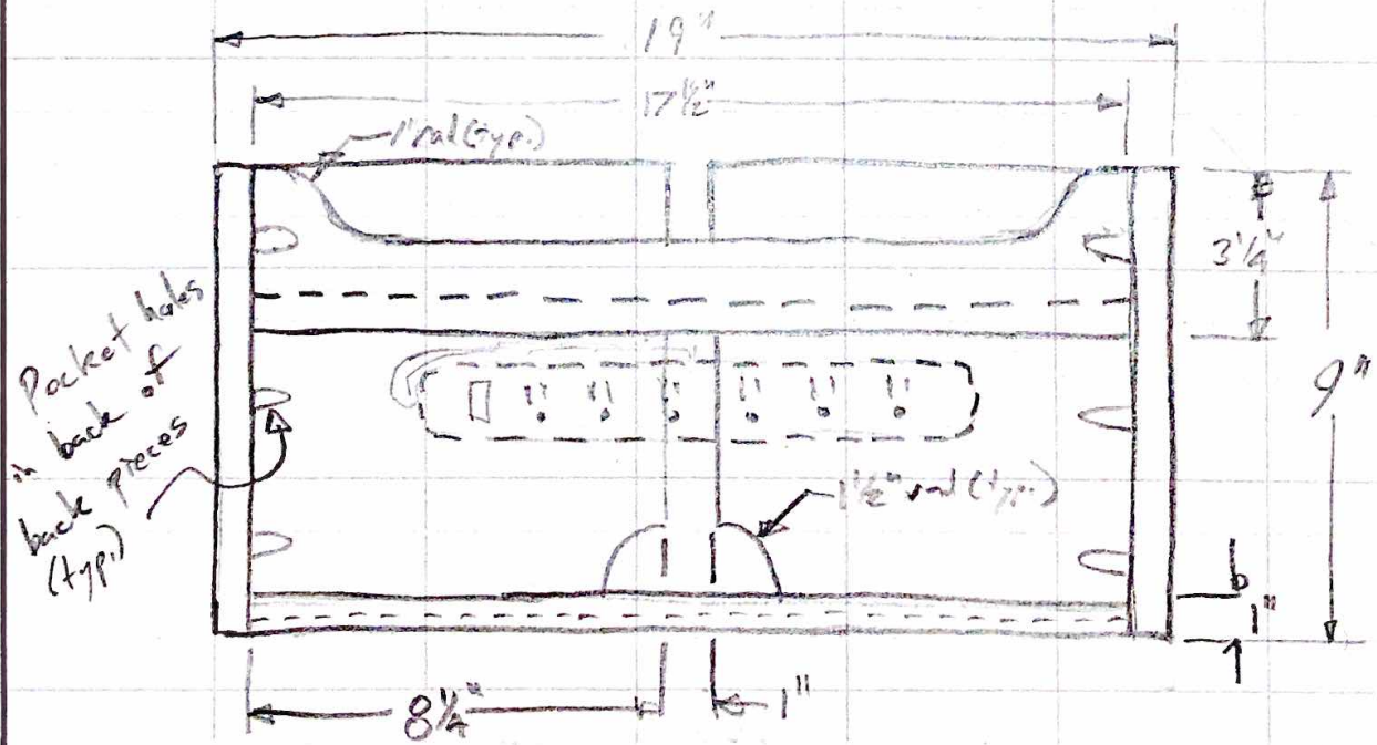
Front Elevation (1:4 scale)
